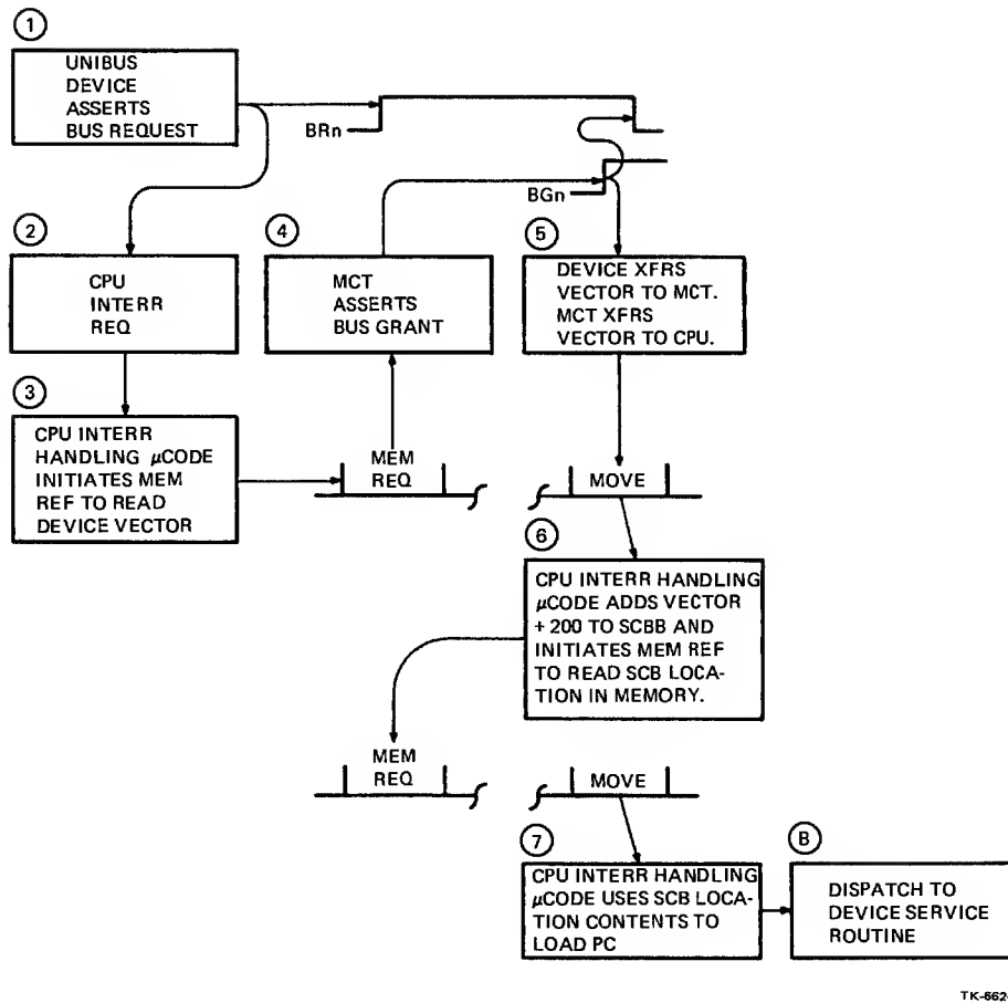
Figure 7-3 UNIBUS Interrupt Request Handling
